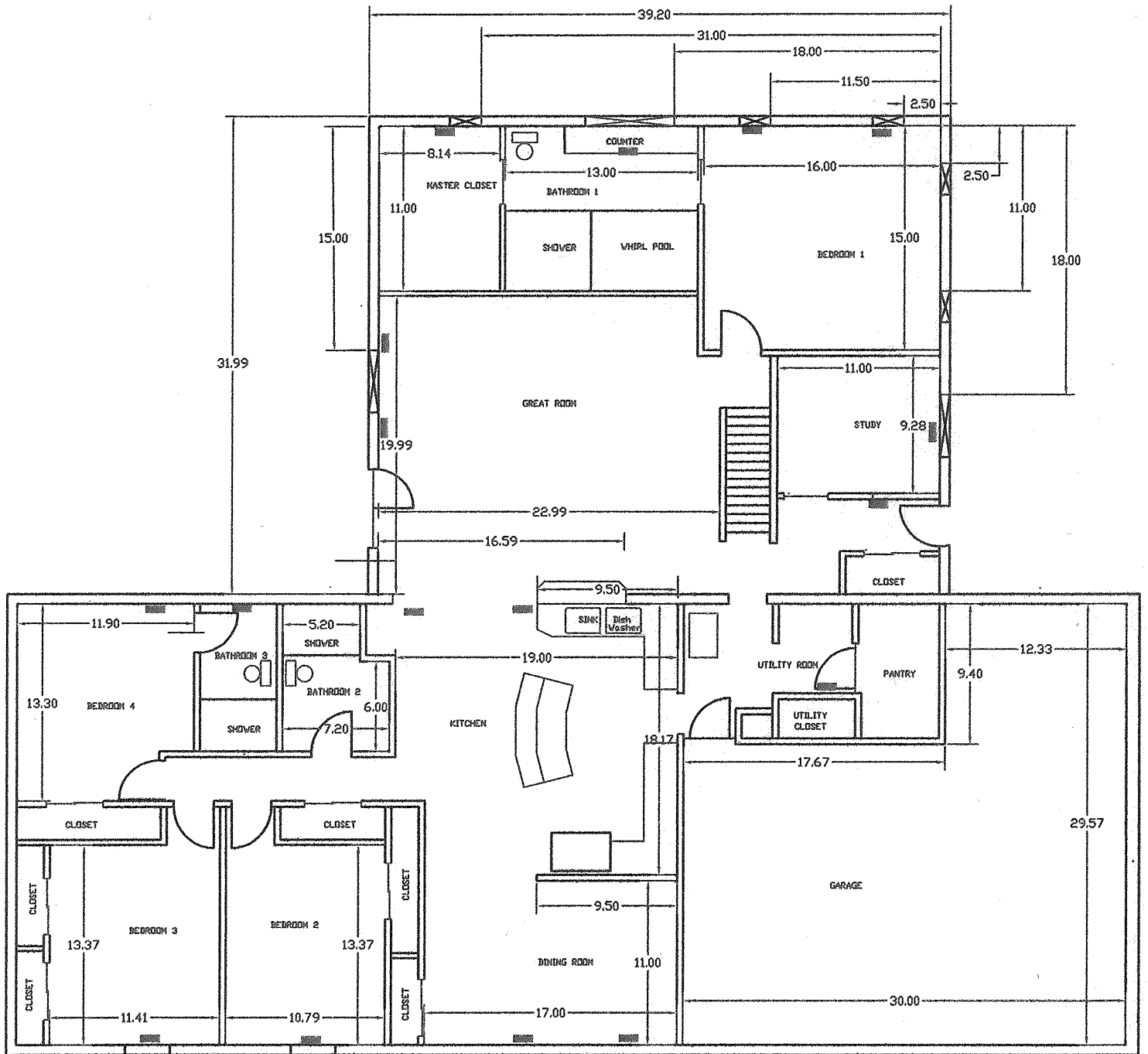
FLOOR PLAN SCALE 1 TO 10
